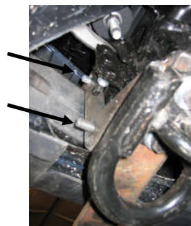
Fig 11 arrows show the threads of the Stiffener Bolt Plate coming through the Top Bracket.
